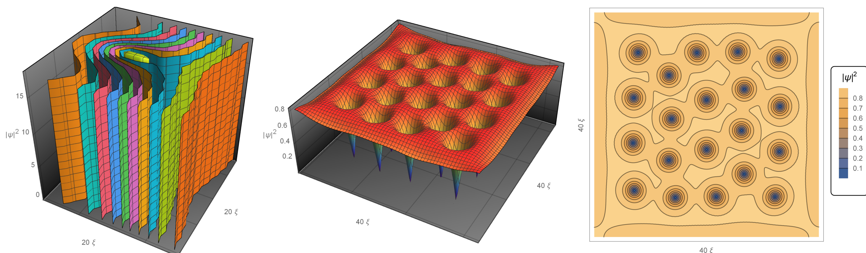
Figure 1: (left) A 3D Example of |\psi|^2 . (Center and right) A 2D example of |\psi|^2 .
